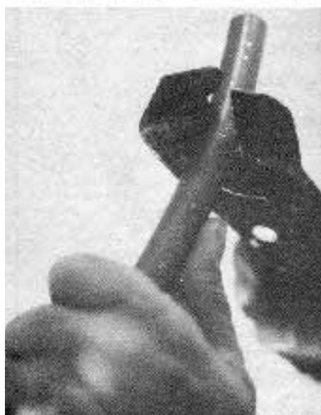
Figure 4. Hand-held cutters cut PB piping to length.
