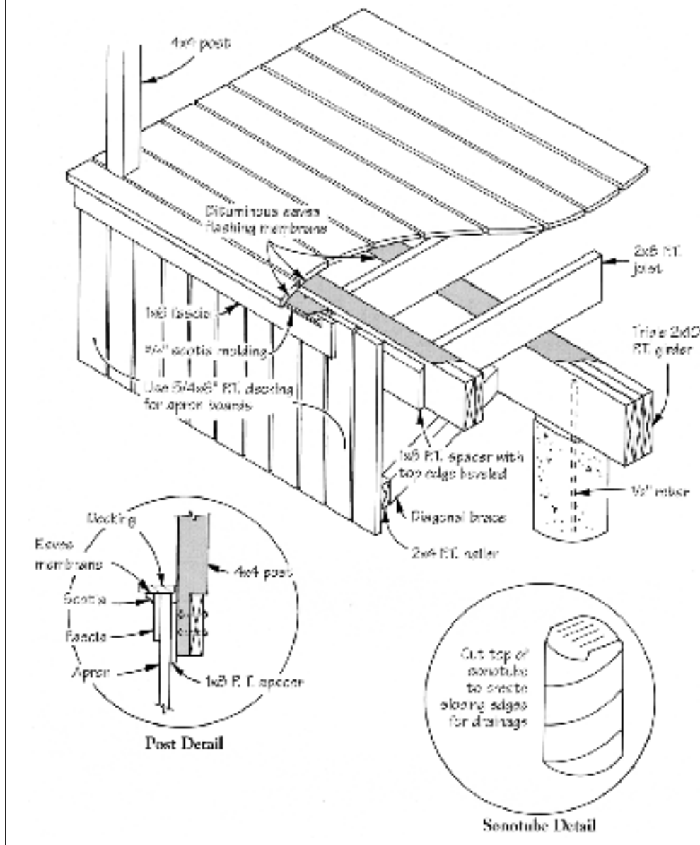
Figure 3. To provide protection against decay, the author covers all sandwich constructions, like the triple 2x girder, with eaves flashing membrane. A beveled 1x spacer directs water through the spaces between the vertical apron boards. Even the sonotube is fashioned to create a watershedding surface at the top.
