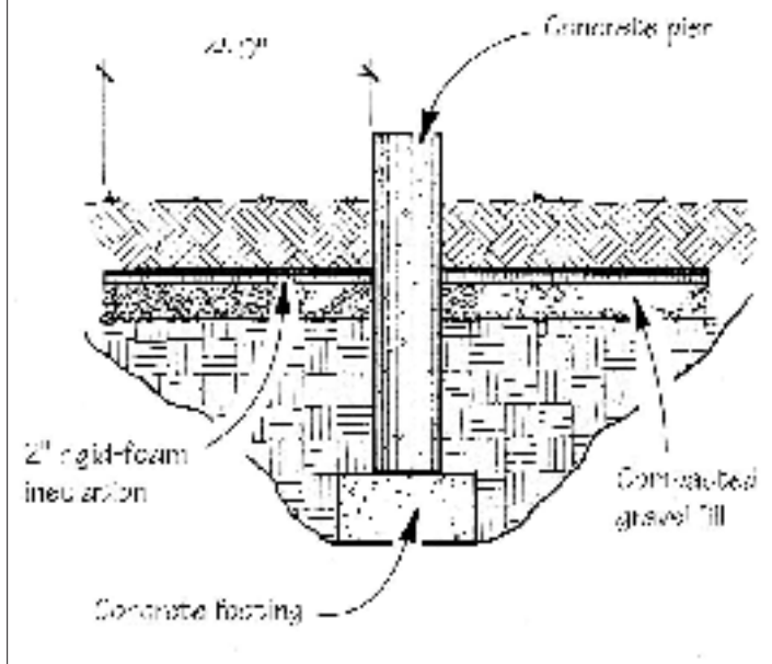
Figure 5. To prevent frost heaving of pier foundations, the author places 2-inch foam horizontally around the piers about a foot below grade.
