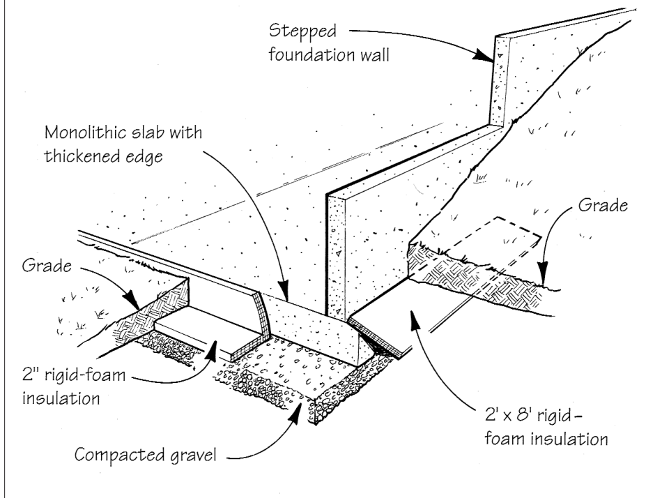
Figure 4. The author protects walk-out basement foundations with foam to avoid having to step down the excavation. A 2x8-foot length of foam board protects the footing of the main wall at the corner where the backfill is shallow.
