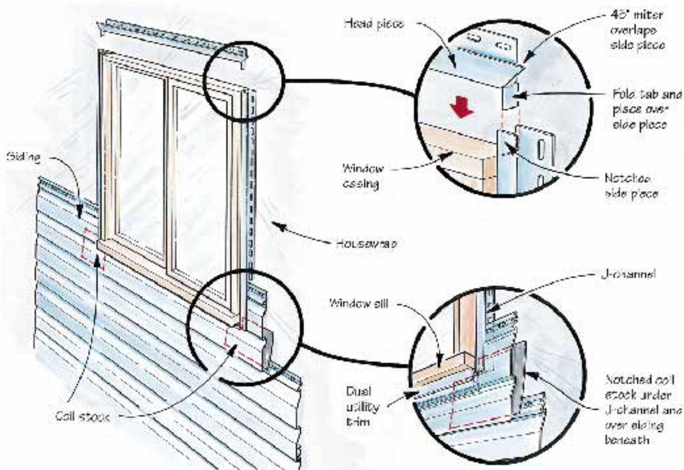
Figure 4. When trimming a window, first run J-channel around all four sides, detailing the head piece as shown. Place a notched piece of coil stock at each corner of the sill to help direct water running down the J-channel over the top of the siding beneath.
