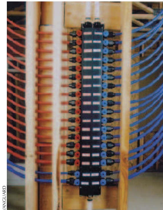
Figure 6. Home-run piping systems use a copper manifold (above) or a plastic manifold (right). Under some codes, the pipe sizing method for home-run manifold systems is different than that used for standard branch systems.
