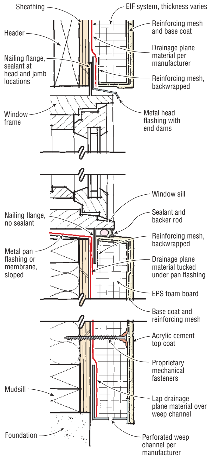
EIF System
