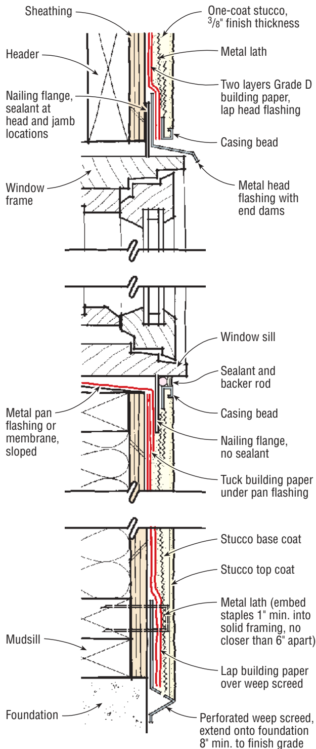
One-Coat System
