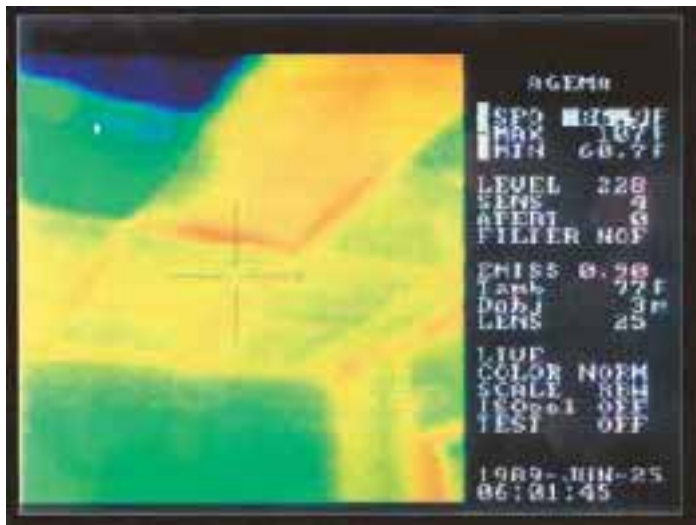
Figure 3. Unfinished galvanized steel roofs may look shiny when new, but they age quickly to become very nonreflective. The infrared thermal scan (above left) shows the drop ceiling (top) at a radiant temperature of almost 90°F under the metal roof of a strip mall building, despite insulation below the roofing. When FSEC researchers applied a reflective coating (right), the building's air-conditioning power use dropped 16%, and tenants reported improved comfort. One tenant even called to thank the landlord for fixing the air conditioner. (He hadn't.)
