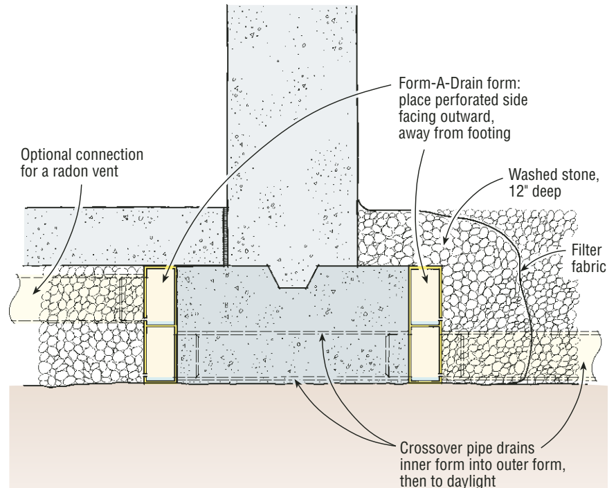
Figure 10. Like any perimeter drain, Form-A-Drain must be protected with clean stone and filter fabric. Note the optional connection for a radon vent.
