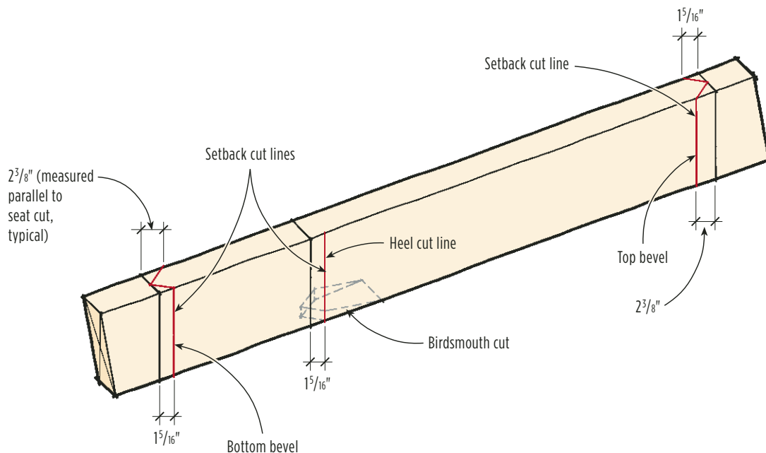
Figure 4. Before cutting the irregular hip rafter to length, the top and bottom plumb marks and the birdsmouth heel cut line must all be shortened, or set back, so that the bevel cuts meet at the hip centerline (below).
