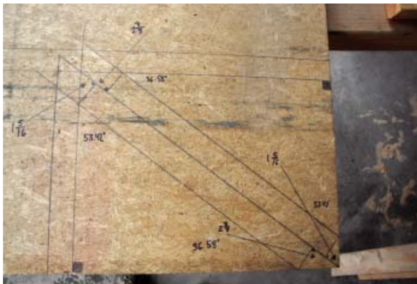
Figure 3. A full-scale drawing of the irregular hip corner helps keep the angles straight. The drawing also gives a quick visual reference for the setback cut lines, which are needed to make the top bevel and birdsmouth cuts meet in the center of the hip.
