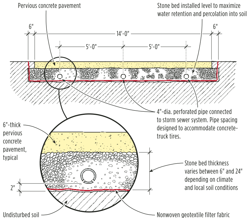
Figure 3. When designing a pervious concrete surface, a free-draining substrate is the key to good performance. The author used 10 inches of stone because the soil beneath had high clay content.
