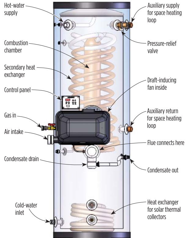
Figure 1. A cutaway drawing of a Vertex heater (above) shows the combustion chamber and secondary heat exchanger coil inside the tank. In the Phoenix model at right, the combustion chamber and secondary heat exchanger are located in the upper part of the tank, with a second heat exchanger for a solar thermal collector below.
