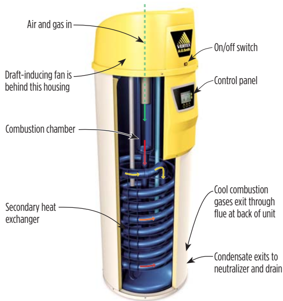
Figure 1. A cutaway drawing of a Vertex heater (above) shows the combustion chamber and secondary heat exchanger coil inside the tank. In the Phoenix model at right, the combustion chamber and secondary heat exchanger are located in the upper part of the tank, with a second heat exchanger for a solar thermal collector below.
