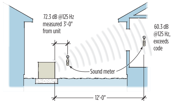
(A) A “quiet” AC condenser that measures 72.3 dB at 3 feet will measure about 60 dB at 12 feet, according to the inverse square rule (doubling the distance yields a reduction of about 6 dB).
